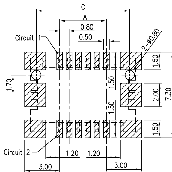
RECOMMENDED PCB LAYOUT GENERAL TOLERANCE \pm 0.05 WITH BOSS
